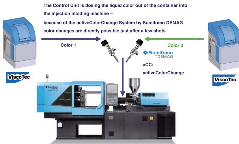
Mixing and dosing for injection molding: ViscoTainer & activeColourChange
