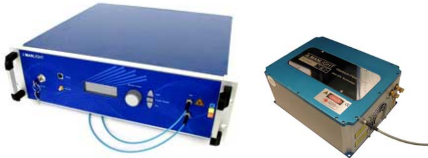
Fiber Laser (pulsed or CW) from Manlight for applications in industrial material processing and test & measurement
