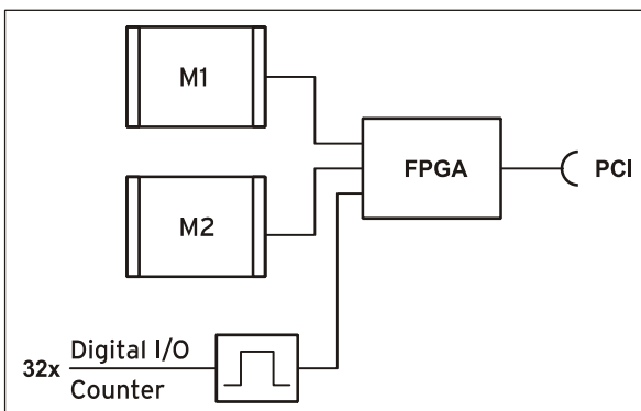
Functional diagram
