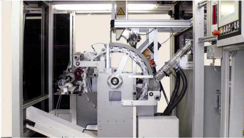
Partial view of „HSC“-High Speed Circular for cylindrical parts (patent pending)
